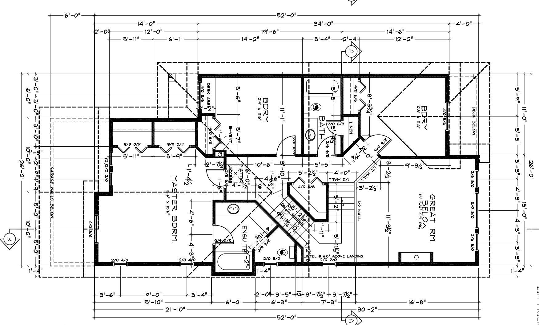
UPPER FLOOR AREA: 896 SQ. FT.
