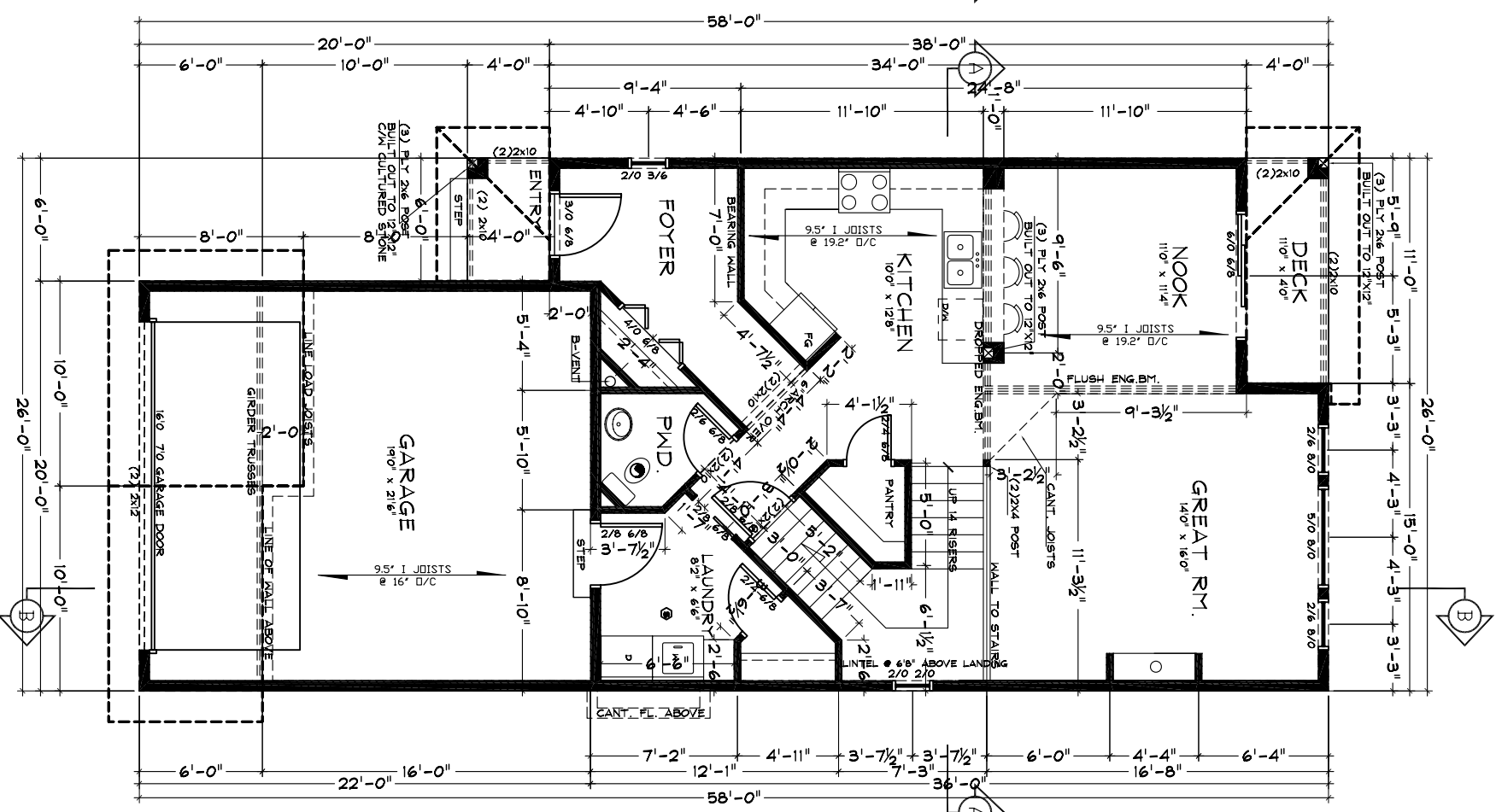
MAIN FLOOR AREA: 905 SQ. FT.
